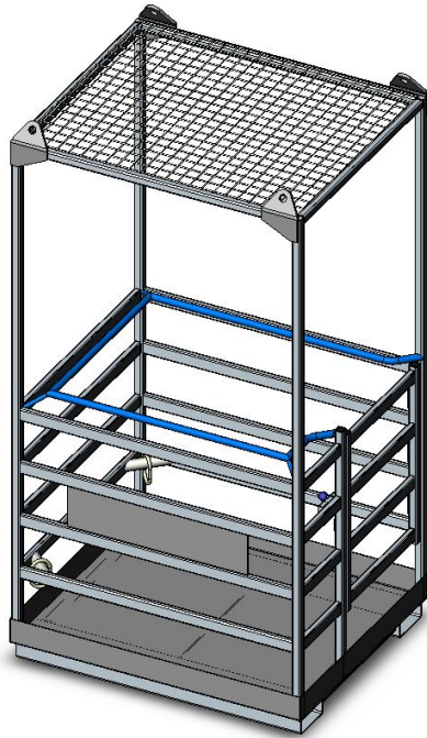
(Lifting Chains not shown)
